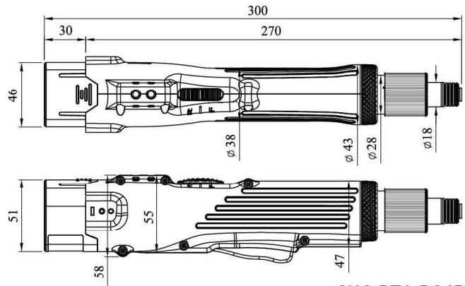
SKC-PTA-BS45
